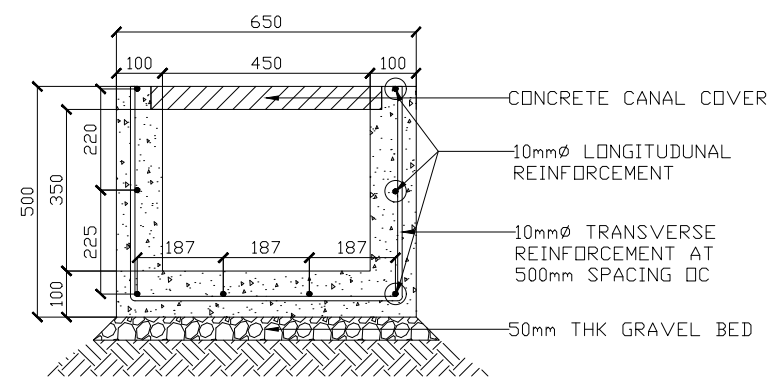
S 503 EMERGENCY ROOM EXTENSION CONCRETE CANAL DETAILS NTS
