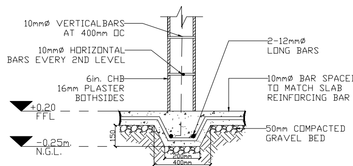
S 504 EMERGENCY ROOM EXTENSION WALL FOOTING 1 (WF1) DETAILS NTS
