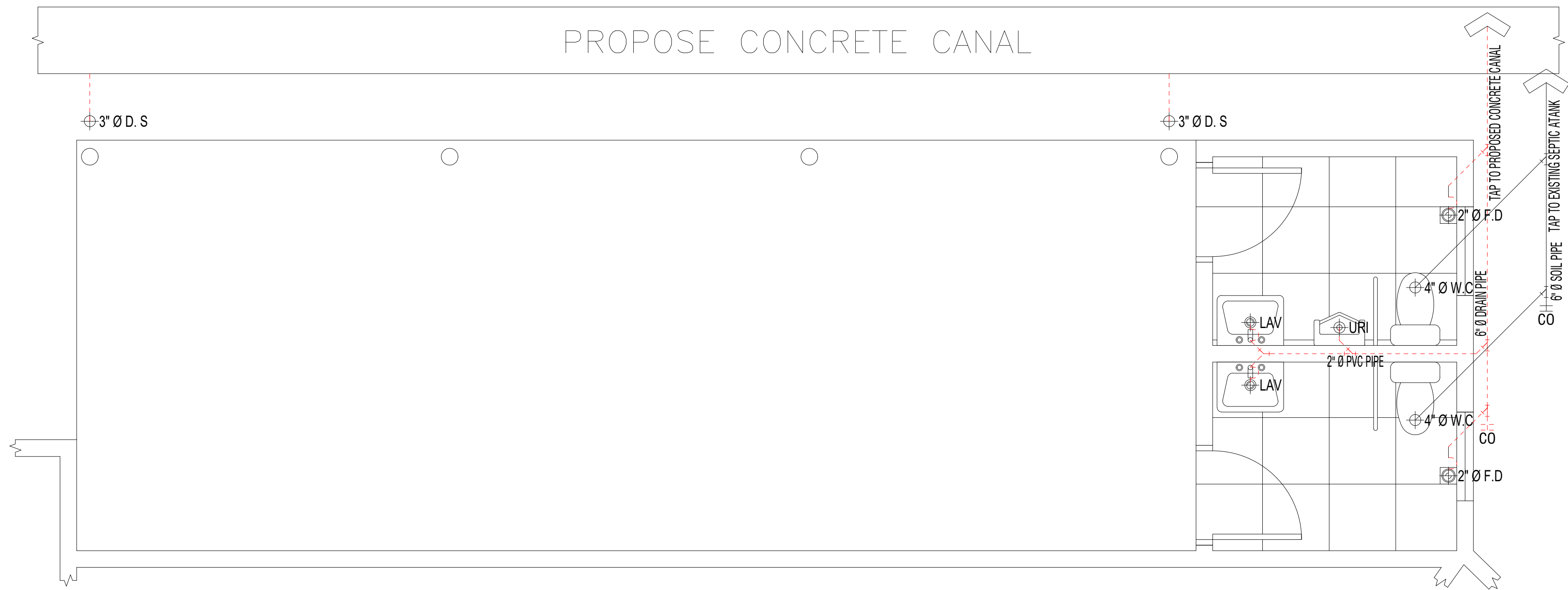
S PAVILION 2 E.R 501 PROPOSED SEWERLINE LAY OUT 1:30M
