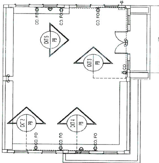
COMPLETION OF FINANCE RECORDS BUILDING E POWERLINE LAY OUT 20' 1:500M
